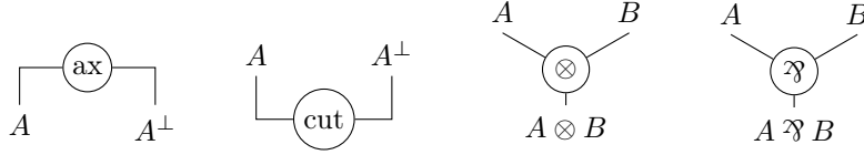
Figure 4.1: Typing of proof structures.
