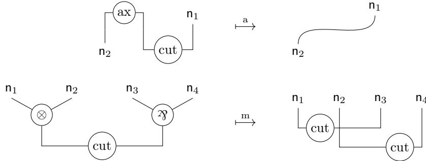
Figure 4.3: Cut elimination steps in multiplicative proof structures
